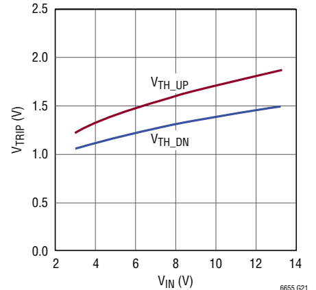
2.5V SHDN Input Voltage Thresholds vs V_{IN}
