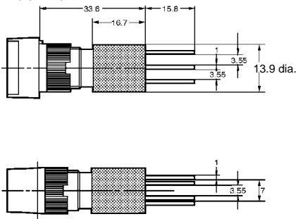
Wire-wrap Terminal A3C-4101
